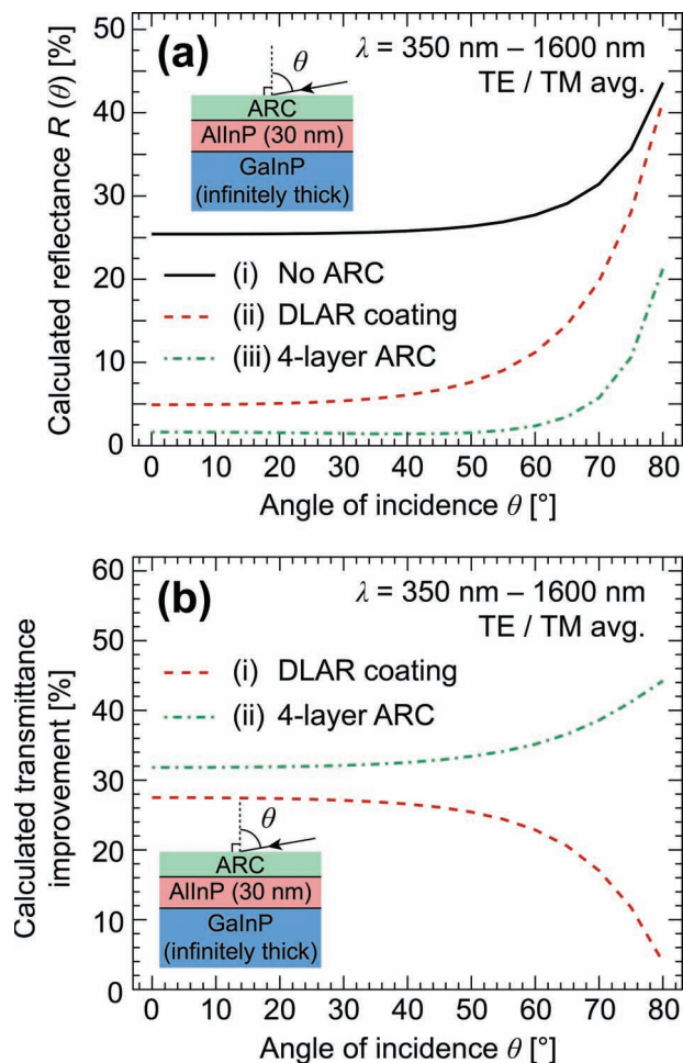
Figure 4. a) Calculated wavelength- and TE/TM-averaged reflectance R(\theta) for AlInP/GaInP structure with (i) no ARC, (ii) DLAR coating, and (iii) four-layer ARC. The AOI-dependent reflectance R(\theta) are equally weighted for the TE and TM mode, and over \lambda = 350\text{--}1600 nm. b) Calculated transmittance T(\theta) improvement due to (i) DLAR coating and (ii) four-layer ARC. T(\theta) = 1 - R(\theta) , assuming no scattering or absorption losses.
