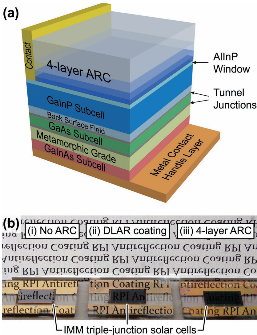
Figure 1. a) Schematic layer sequence of an inverted metamorphic (IMM) triple-junction solar cell with four-layer ARC. b) Photograph of three IMM solar cells with (i) no ARC, (ii) DLAR coating, and (iii) four-layer ARC.
